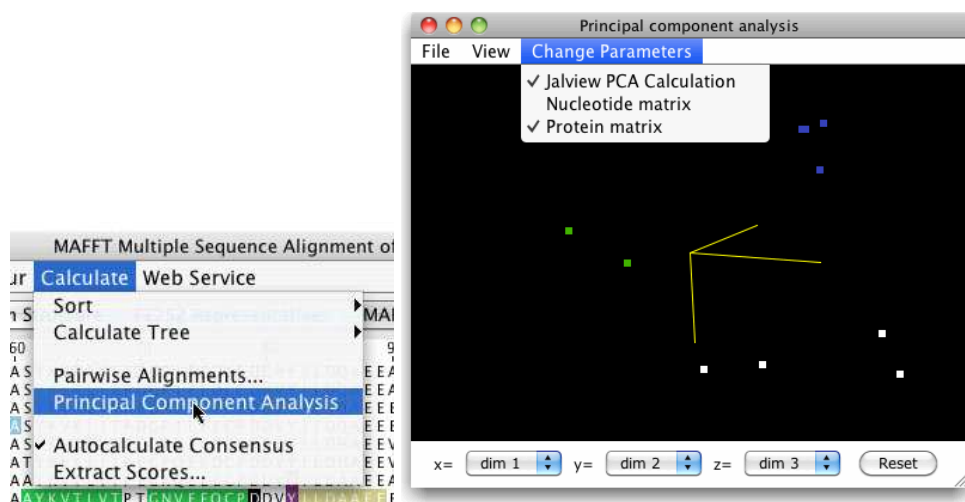
Figure 2.7: PCA Analysis.
